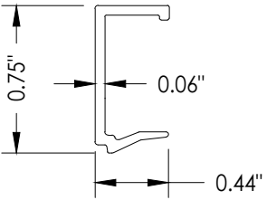
2 GLAZING BEAD
