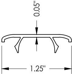
7 SASH STOP
