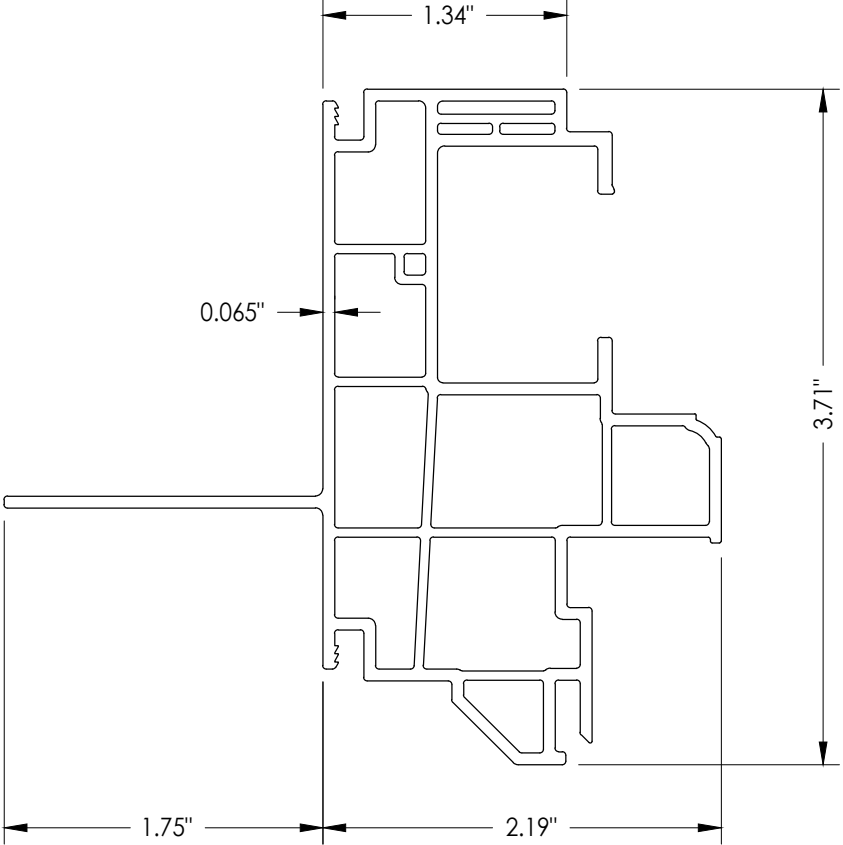
1 FRAME
