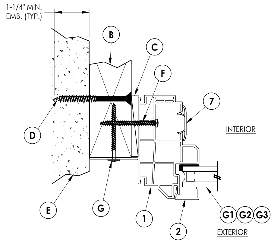
1 HORIZONTAL CROSS SECTION 2 Shown w/ 2X Buck Construction
