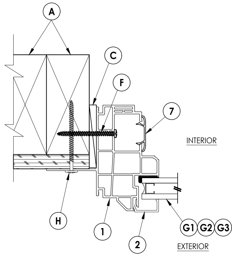
2 HORIZONTAL CROSS SECTION 2 Shown w/ Stud Construction
